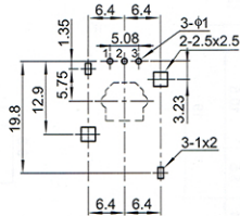
Recommend PCB Layout Jack Top View
