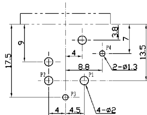
Dimensions of PC board holes (Comment)
