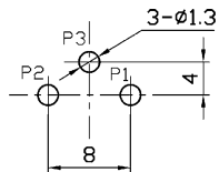
Dimensions of PC board holes (Commend) Top View (t=1.6mm) ⊗
