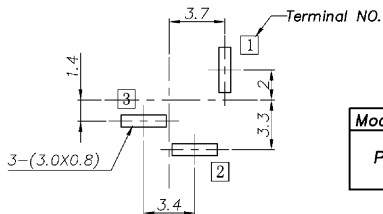
P.C.B Layout (Copper-sided view)
