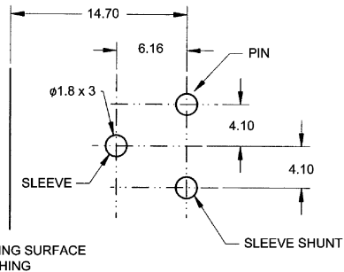
RECOMMENDED PANEL LAYOUT (COMPONENT SIDE)
