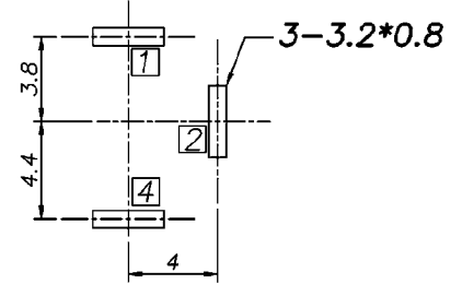
P. C. B Layout (Copper-sided view)
