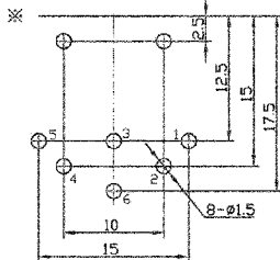
Dimensions of PC board holes (Comment)
