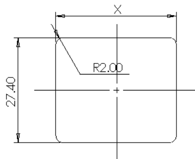
PANEL CUT-OUT
